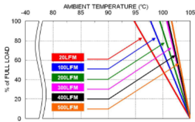
43RHK03-110S24W Derating
