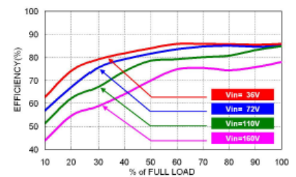
43RHK03-110S24W Efficiency vs. Output Load
