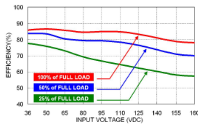
43RHK03-110S24W Efficiency vs. Input
